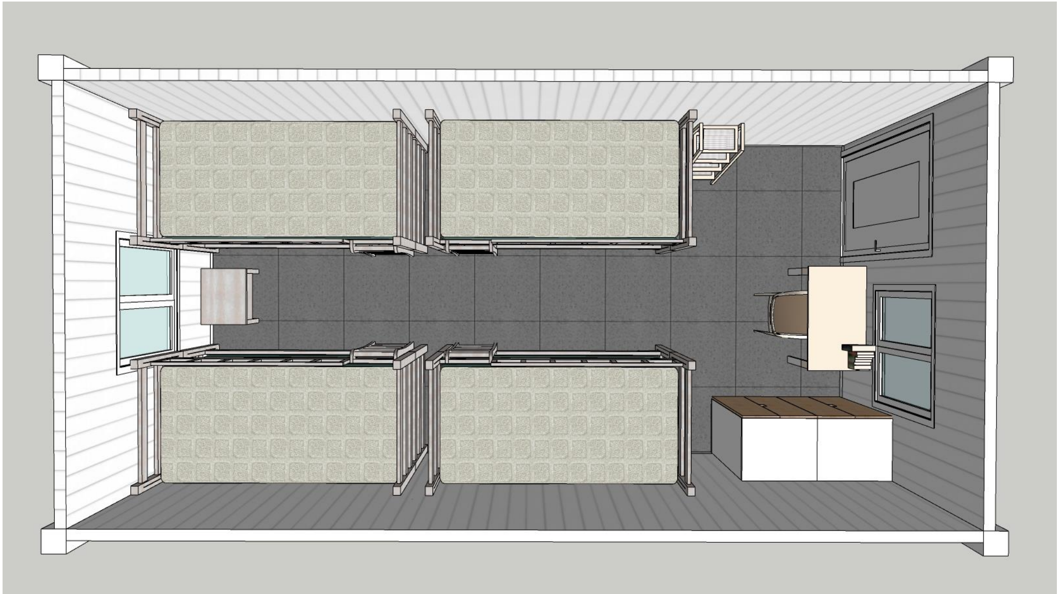
Type-05, Container House Layout for 8 people
